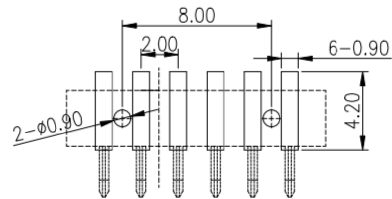
RECOMMENDED P.C.B LAYOUT TOP VIEW (.XX±0.05)
